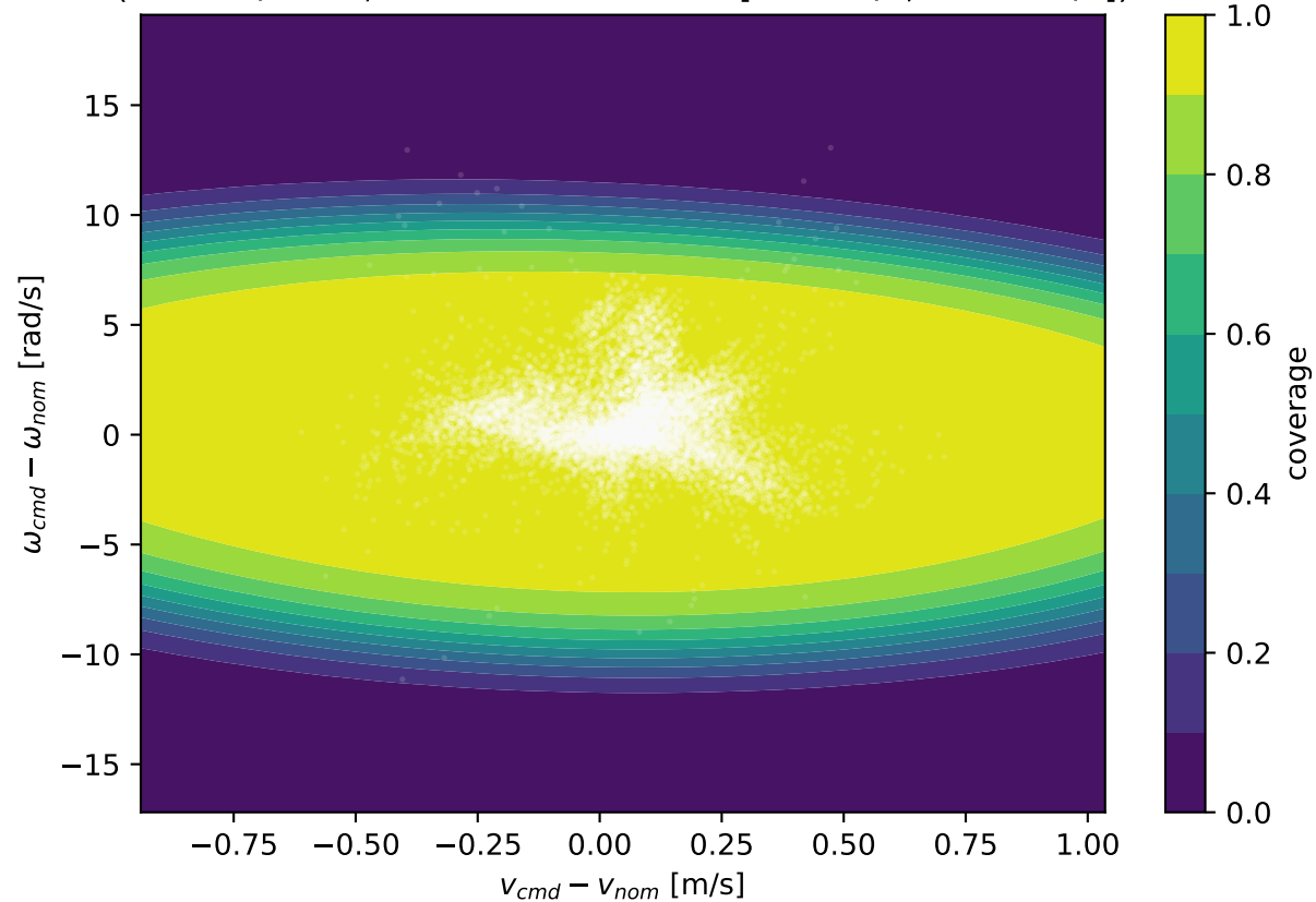
Residual coverage vs command offset (0 = off / OOD; state fixed at mean [0.55 m/s, 0.50 rad/s])
